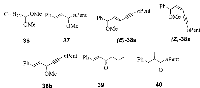
Figure 2. Structure of compounds 36 – 40 .
